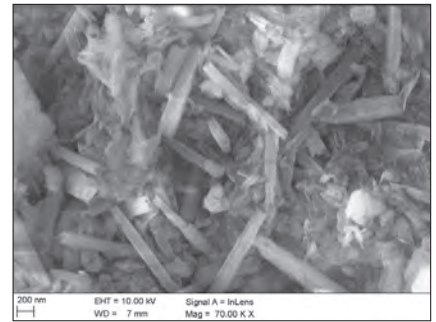
Rys. 1 Widok mikroskopowy SEM haloizytu Dunino Fig. 1 SEM picture of Halloysite from “Dunino” mine
