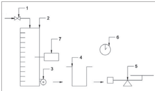
Fig. 3. Diagram of test stand 1 – valve, 2 – tank, 3 – cylindrical flow regulator, 4 – measuring vessel, 5 – scales, 6 – stopwatch, 7 – thermometer
