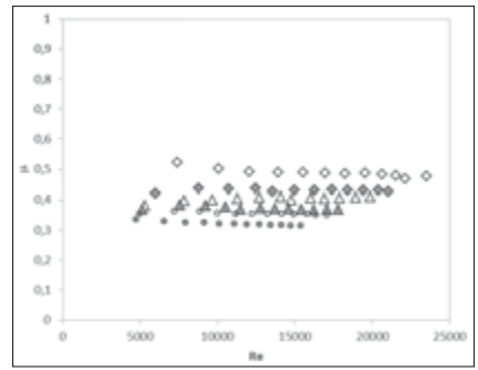
Fig. 4. A comprehensive chart of the dependence of the value of the discharge coefficient \mu on the Reynolds number for a cylindrical flow regulator. ( \diamond 3d with core hole; \bullet 3d without core hole; \triangle 4d with core hole; \cdot 4d without core hole; \square 5d with core hole; \square 5d without core hole)
