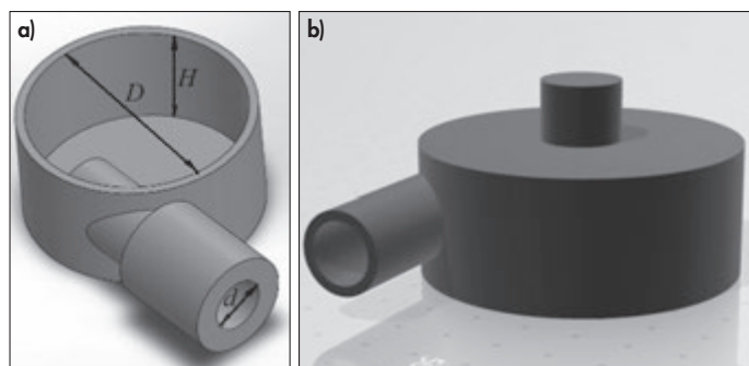
Fig. 1. Cylindrical vortex regulators [11]: a) classical construction with symbols, b) with a core-hole
