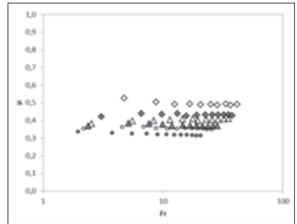
Fig. 5. A comprehensive chart of the dependence of the value of the discharge coefficient \mu on the Froude number for a cylindrical flow regulator. ( \diamond 3d with core hole; \bullet 3d without core hole; \triangle 4d with core hole; \cdot 4d without core hole; \square 5d with core hole; \square 5d without core hole)
